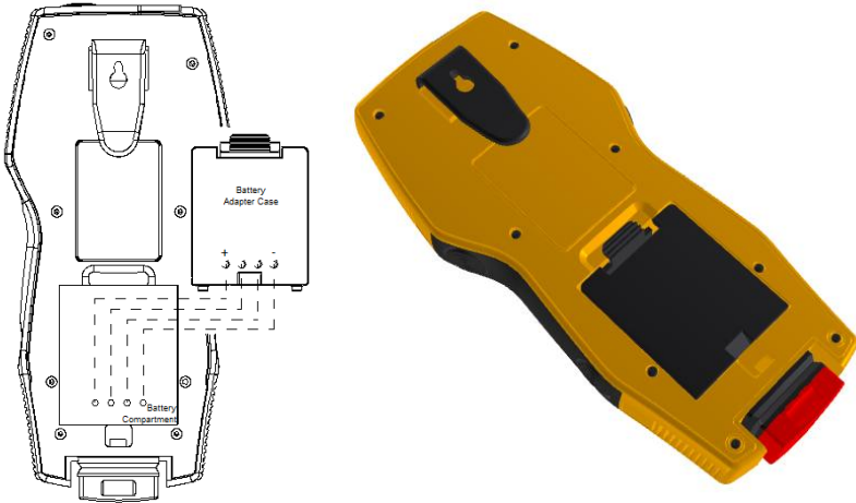
Figure 4. Inserting Battery
